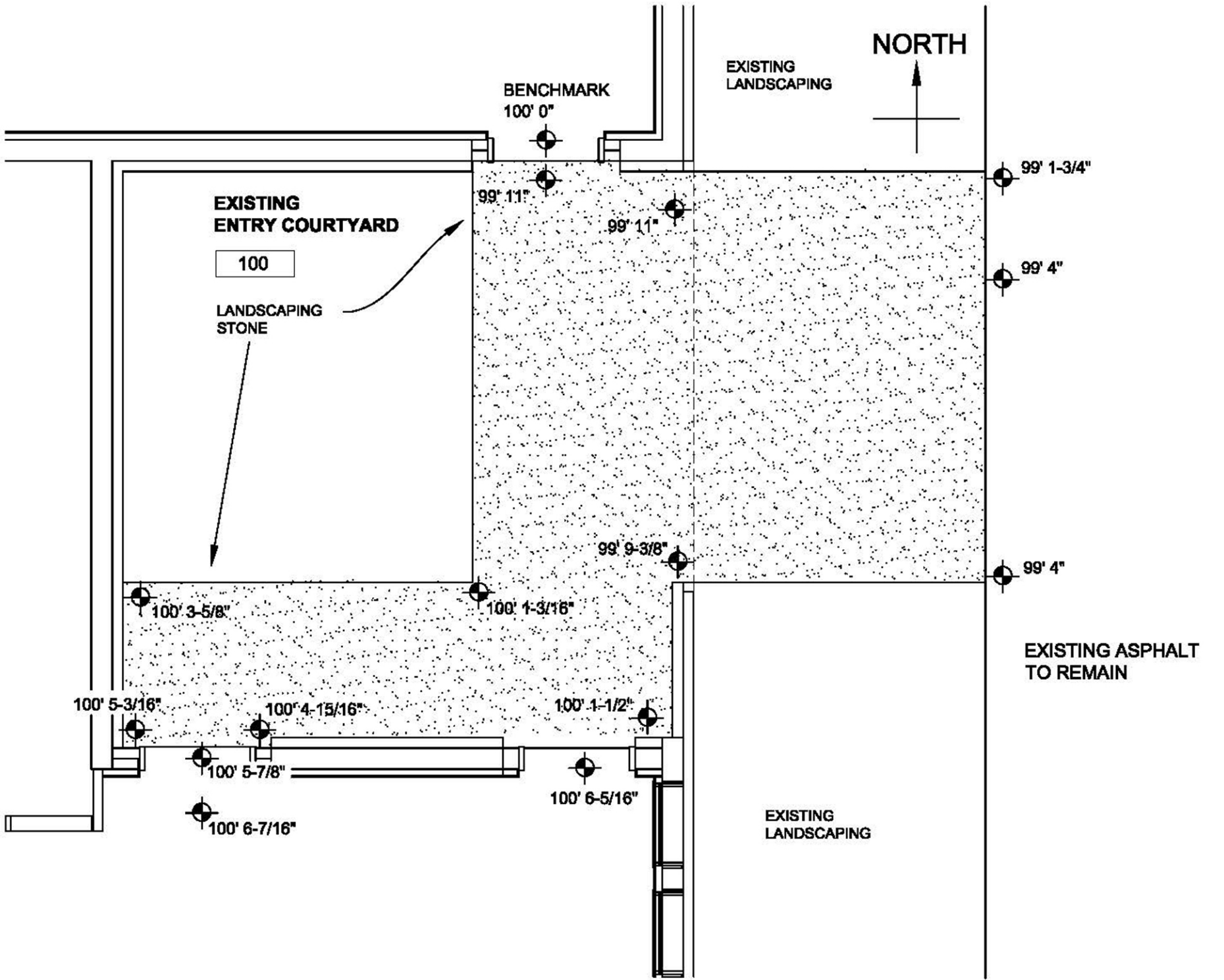
SPOT ELEVATIONS - EXISTING
