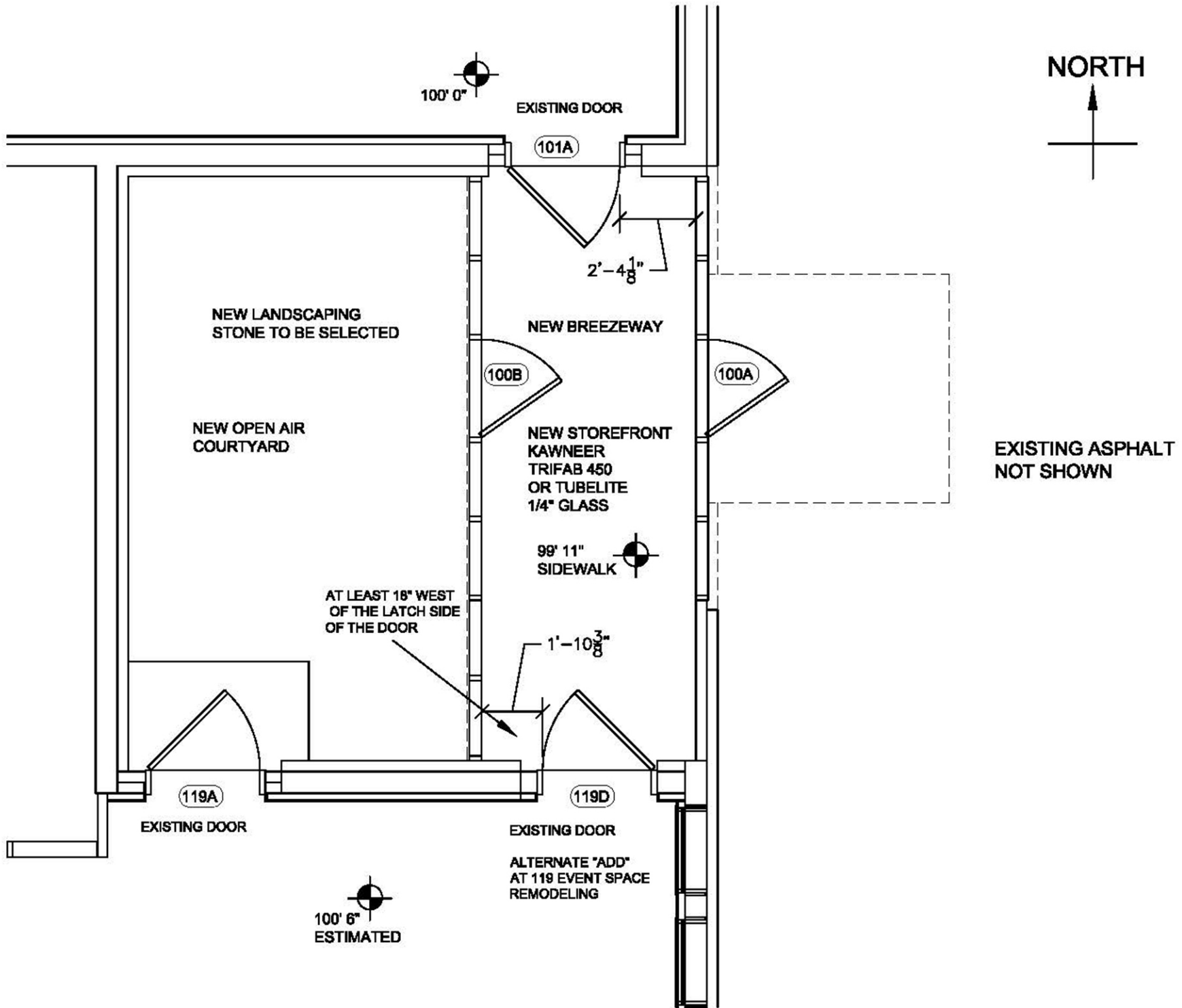
STOREFRONT PLAN VIEW
