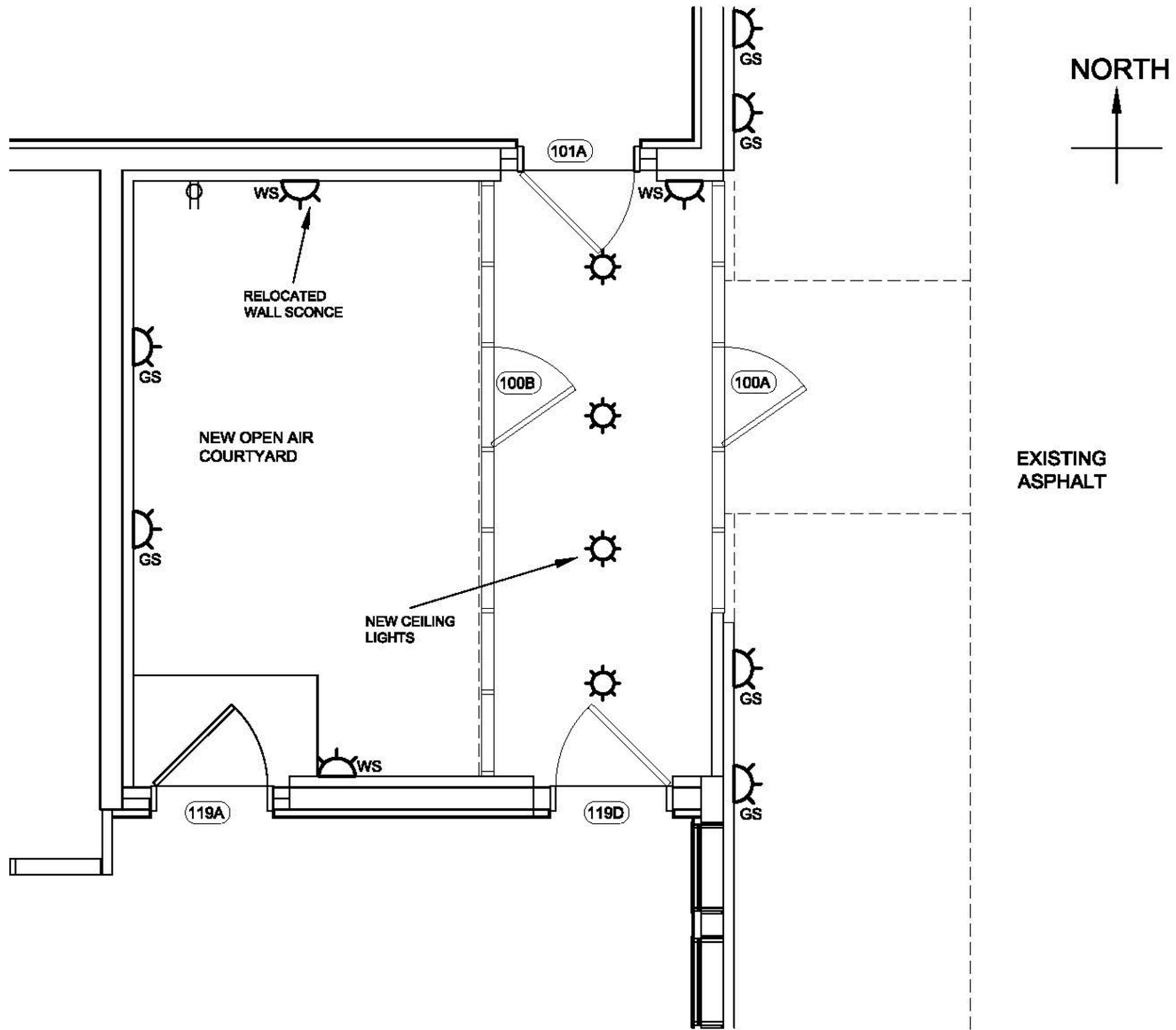
NEW ELECTRICAL PLAN
